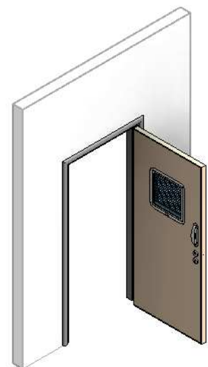
Fig.2 - 3D view of the Kingsway Solo Doorset in the open position. The family provides the ability to view the door in closed or open positions in 3D views without the need for creating additional family types.
