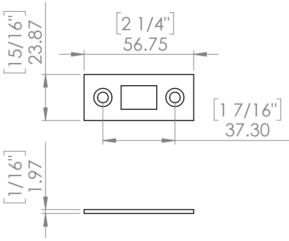
Frame Lock Keep Plate
