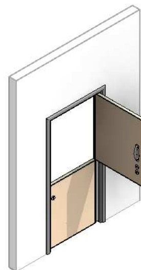
Fig.2 - 3D view of the Kingsway Stable Doorset in the open position. The family provides the ability to view the door in closed or open positions in 3D views without the need for creating additional family types.
